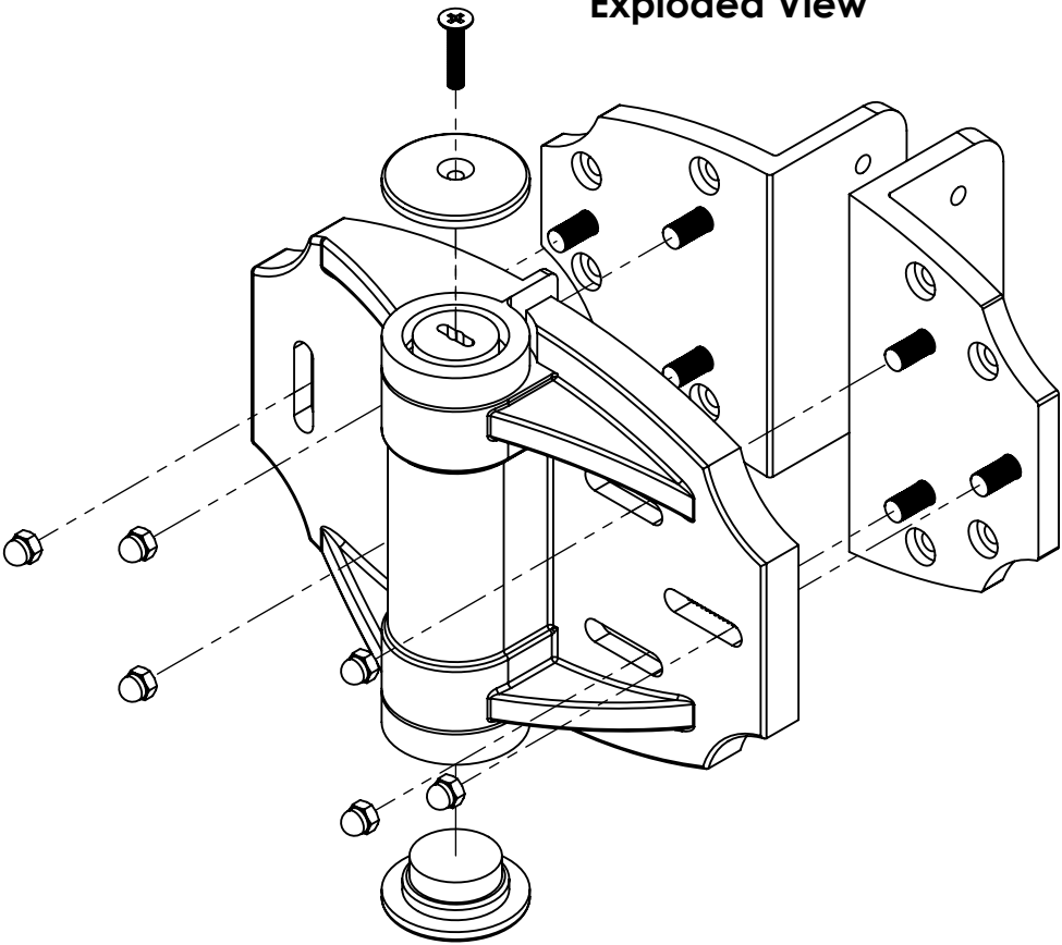
Exploded View
