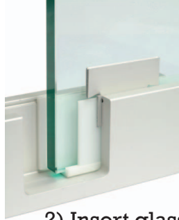
2) Insert glass and aluminium wedge - check alignment
