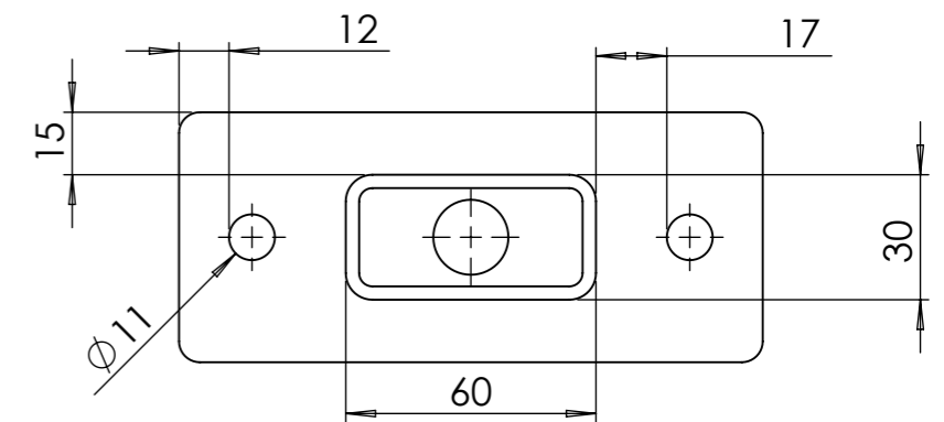
EXAMPLE OF BASE PLATE FIXTURE
