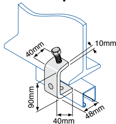
Beam Clamp
