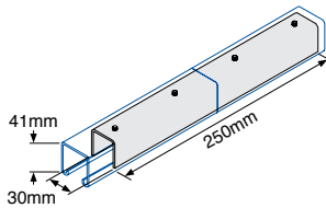
Internal Connector
