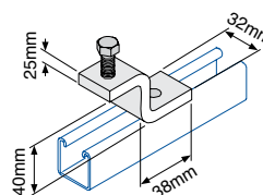
'Z' Beam Clamp
