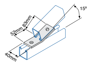
External Obtuse 45° Angle Bracket
