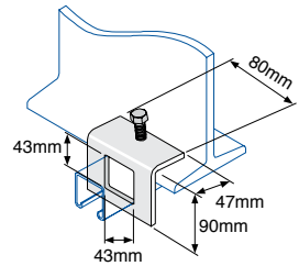
Beam Clamp
