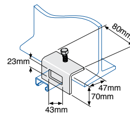
Beam Clamp
