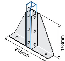
Single Delta Plate
