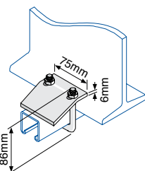
Beam Clamp 'U' Bolt
