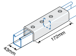
External Connector
