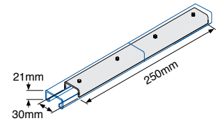
Internal Connector
