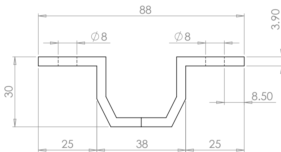
DETAIL A SCALE 1 : 1
