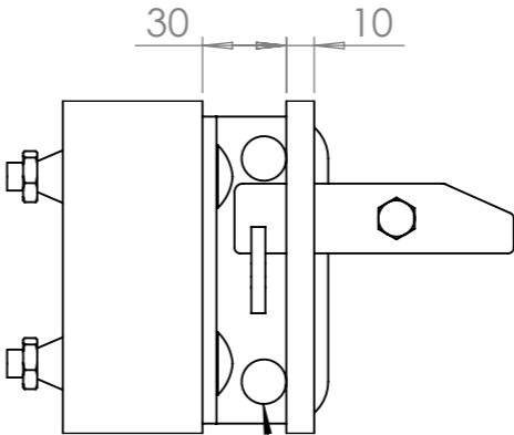
DETAIL A SCALE 1 : 3
