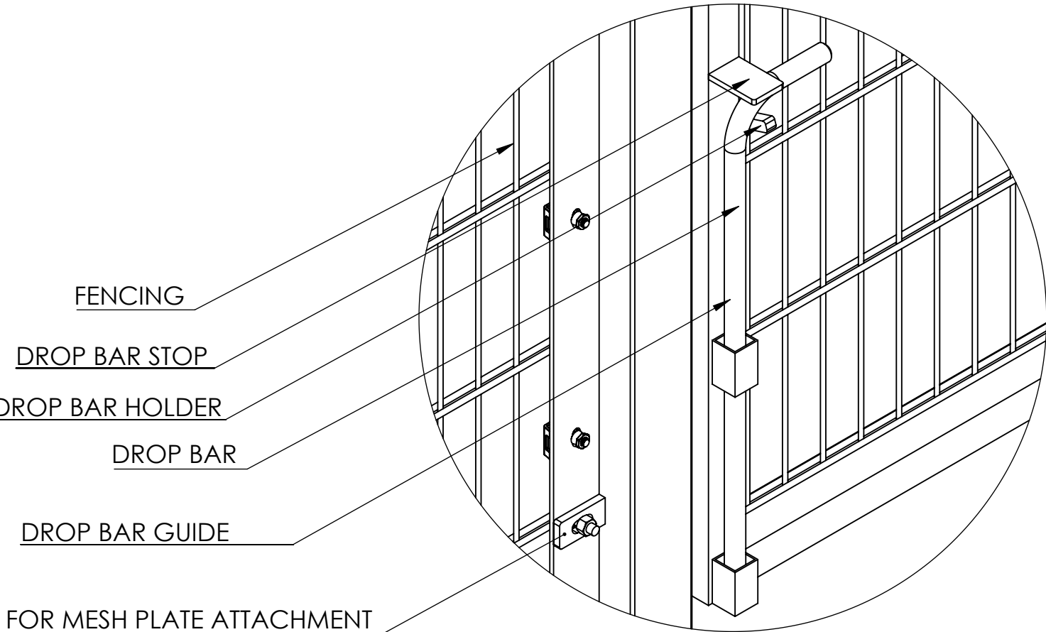
Back View of Drop Bar and Mesh Attachment Plate. Mesh Plate & Fittings sold separately
