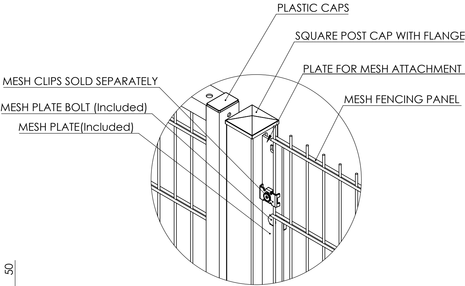
Gate & Fence Attachment Example This Can Be Achieved Using The Fixing Which Are Sold Separately.
