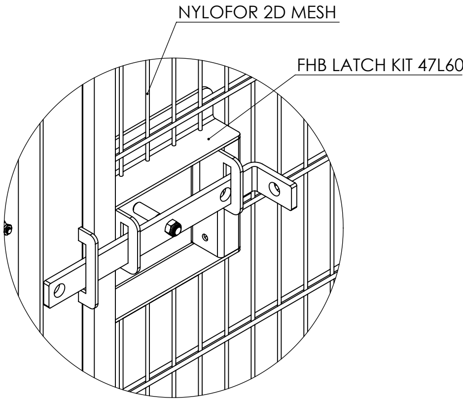
Slide Latch With Padlock Holes & Removable Handle As Standard. (Padlock Not Included)
