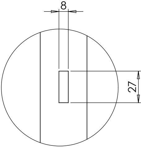
SLOTS SCALE 1 : 2
