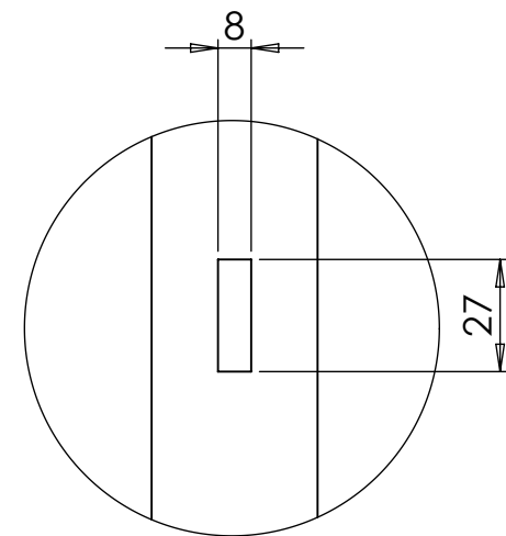
SLOTS SCALE 1 : 2
